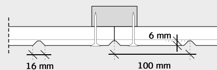
CROSS SECTION v-line 2way 6
