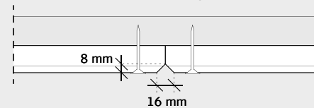
LONGITUDINAL SECTION v-line 2way 10, 6 and blank
