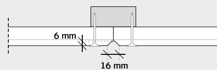
LONGITUDINAL SECTION v-line 2way 10, 6 and blank
