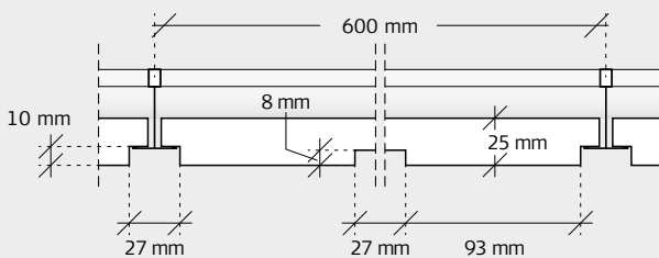
CROSS-SECTION: Troldtekt® Tiles 5, T24
